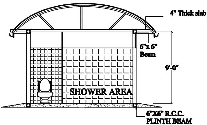
SECTION y-y
